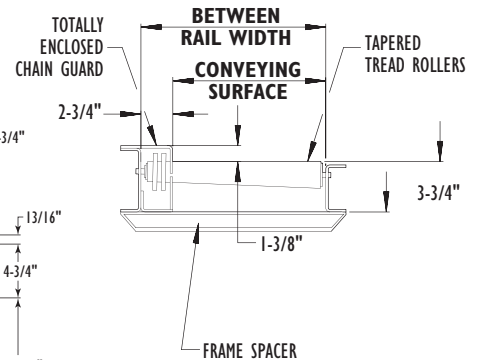
SECTION Y-Y
