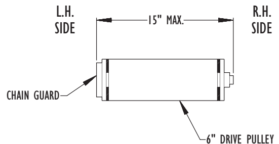
SECTION Y-Y
