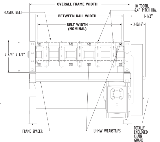
SECTION X-X
