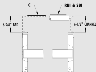
SECTION "X-X"
